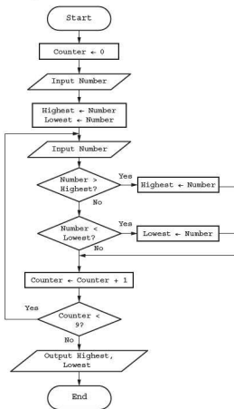
Figure 9.15 A readable algorithm
