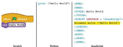
Figure 11.1 Programs to display
