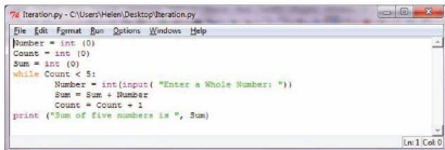
Figure 11.17 Python repetition program
