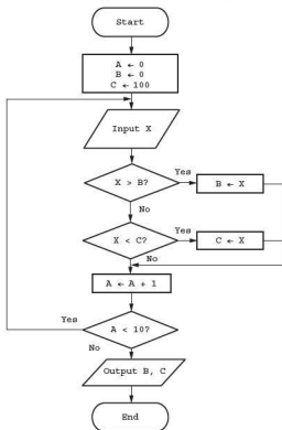
Figure 9.11 Flowchart to trace
