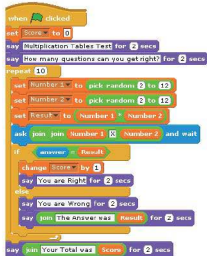
Figure 7.1 Program written in Scratch
