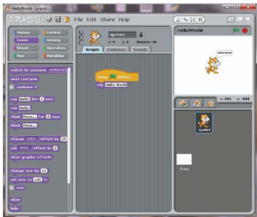
Figure 11.4 Scratch IDE
