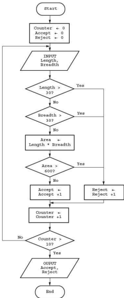
Figure 9.17 Flowchart
