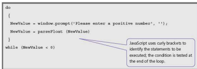
Figure 11.23 Unknown number of repetitions, at least one completed
