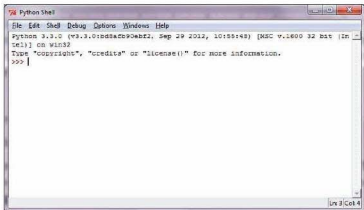
Figure 7.5 Python IDE
