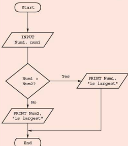
Figure 9.4 Flowchart
